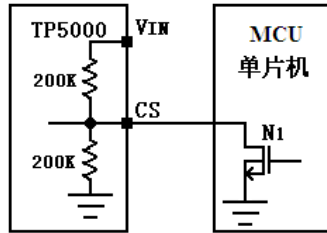
Figure 8 switch controlled by external LiFePO4 state of charge and stop state
