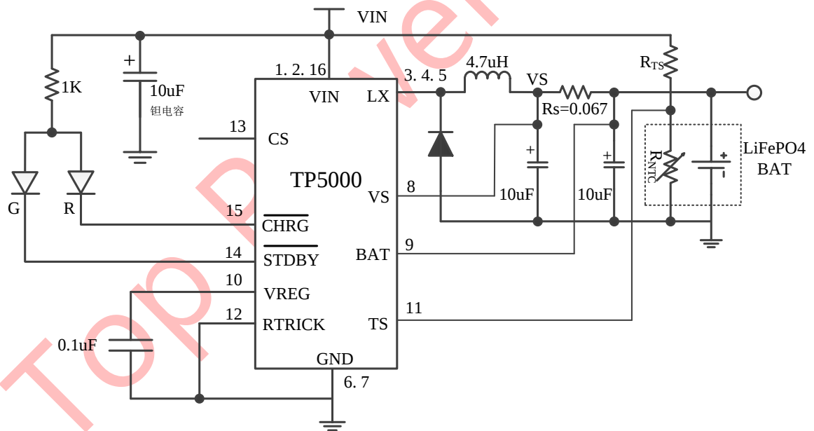
Figure 2 TP5000 3.6V LiFePO4 battery charging 1.5A (150MA prefill) Application Diagram
