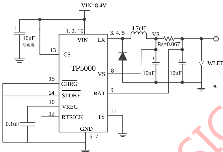
Figure 14 TP5000 The two connected lithium battery drive 5W LED Application Diagram (The RTRICK pin unconnected)
