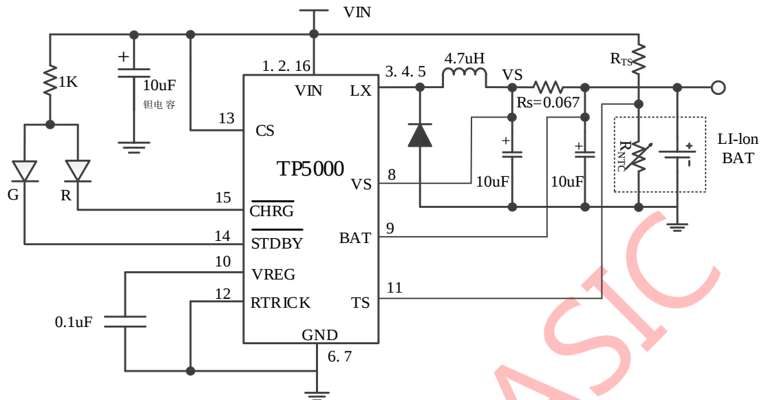
Figure 1 TP5000 4.2V lithium-ion battery charging 1.5A (150MA prefill) Application Diagram
